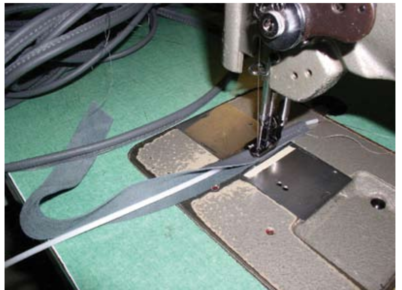
Fabricating cording.
